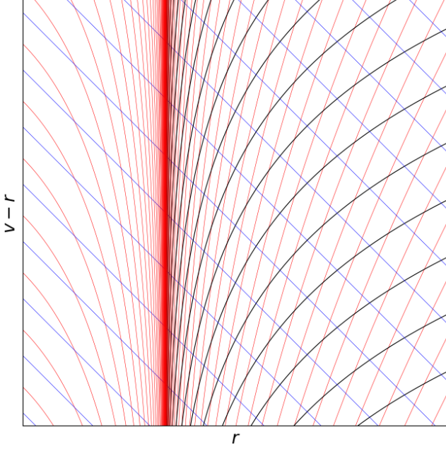
FIG. 3. Level sets of the stationary Schwarzschild time coordinate t (black) plotted on an ingoing Eddington–Finkelstein diagram. Outgoing (red) and ingoing (blue) null rays are shown. The Schwarzschild slices t = \text{const} tilt upward and accumulate along a single generator of \mathcal{H}^+ , becoming asymptotically tangent to it. Although this image uses the stationary t coordinate, the asymptotic piling-up is a generic consequence of the Null–Temporal Degeneracy Theorem and Lemma 1: any temporal function adapted to an exterior observer [3] must degenerate in exactly this way, with all late-time slicings converging on the same null generator.
