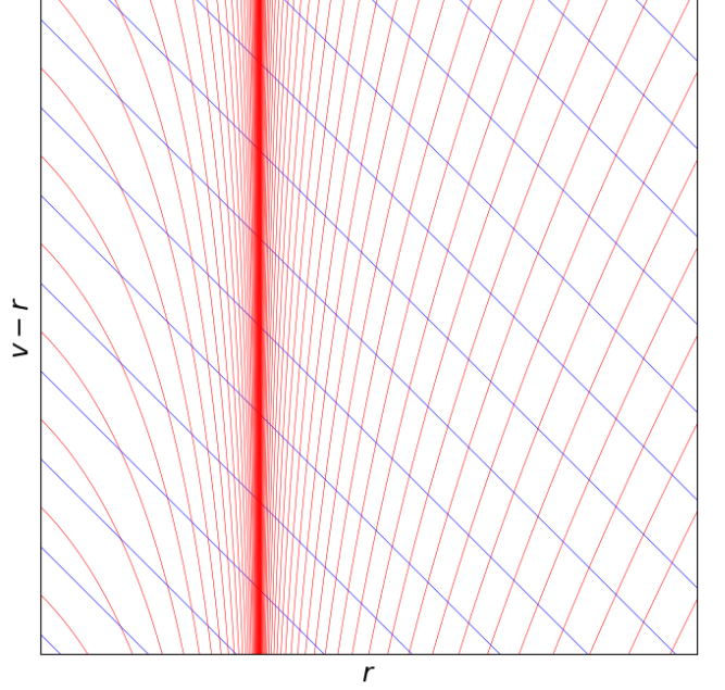
FIG. 1. Null structure near the Schwarzschild event horizon in ingoing Eddington–Finkelstein coordinates (v, r) . Outgoing null rays (red) and ingoing null rays (blue) are shown. The vertical line at r = r_h represents a null generator of \mathcal{H}^+ . Its apparent “length” in the diagram is purely topological : all points along the generator are metrically coincident, with zero invariant temporal or spatial separation along the null direction. Distinct horizon-crossing events correspond to distinct manifold points but share the same null geometric location; the vertical extent depicted here therefore does not represent metrical duration or physical extent in the Lorentzian geometry.
