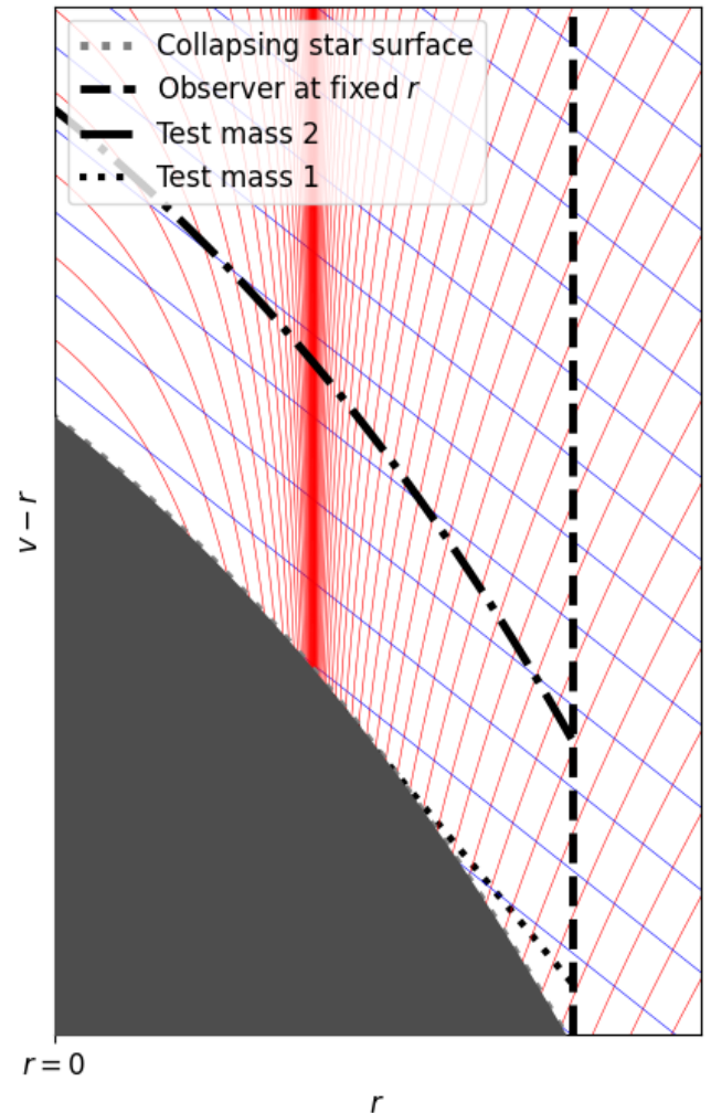
FIG. 2. Radial gravitational collapse in ingoing Eddington–Finkelstein coordinates. The dotted grey curve represents the collapsing star's surface. The dashed curve is an external observer held at fixed radius r > r_h . Test mass 1 (dotted) reaches the stellar surface prior to horizon formation. Test mass 2 (dash-dot) is released later, and its ingoing null signal (blue grid) no longer intersects the collapsing surface. Outgoing null rays (red grid) emitted in the exterior region reach the observer, who therefore only ever sees the star and infalling masses asymptotically approach r_h . The shaded region indicates the stellar interior.
